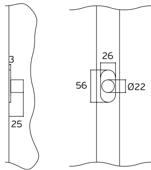
Strike plate
