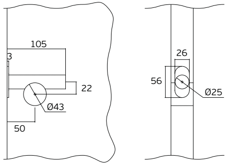
Lock cut-out
